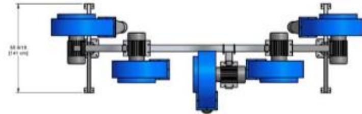
Five motor configuration utilizing (H815406) Blower Support Bracket for center blower
